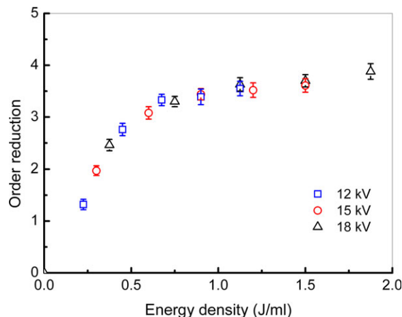
Figure 7. Orders reduction in terms of the plasma energy density under the applied voltage from 12 to 18 kV, water conductivity of 3.5 \mu\text{S/cm} and cell initial density of 6 \times 10^6 \text{ cfu/mL} .
