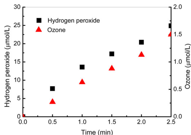
Figure 16. Production of aqueous hydrogen peroxide and ozone under 3.5 \mu\text{S/cm} .
