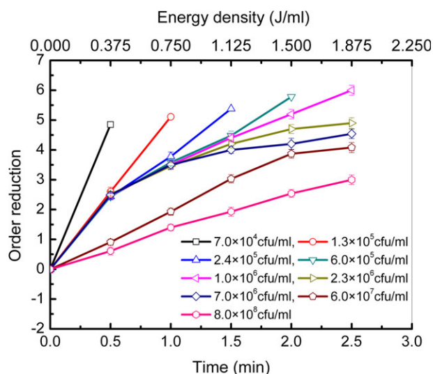
Figure 8. Effect of the initial cell density on disinfection efficiency under 18 kV and 3.5 \mu\text{S/cm} .
