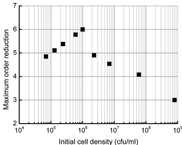
Figure 9. The maximum value of the order reduction in terms of the initial cell number density when the energy density is less than 2 \text{ J/mL} .
